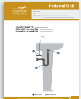
Pedestal Sink
