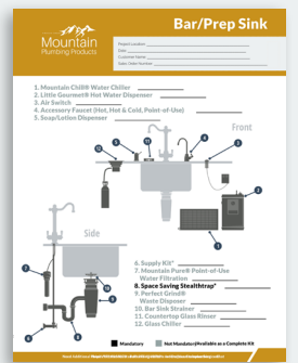
Bar/Prep Sink
