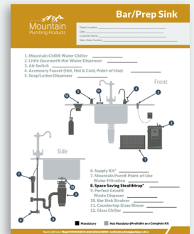
Bar/Prep Sink
