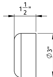
MT314X OPTIONAL HIGH BOX FLANGE
